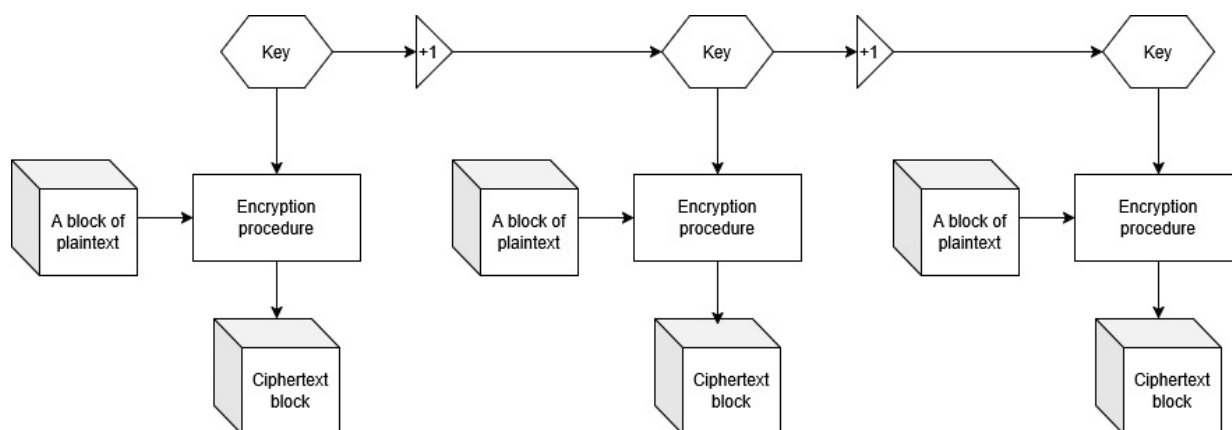
Figure 4 – Cryptoalgorithm
