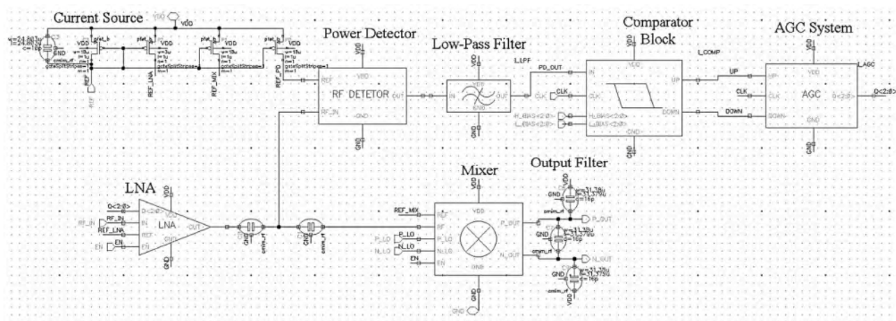
Figure 2.1 – The proposed design of receiver
