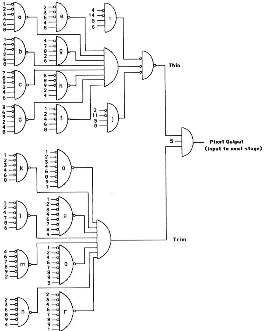
FIG. 8. The realization of the thinning, restoring, and trimming operations.
