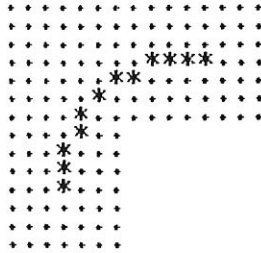
FIG. 1. The bias skeleton. The algorithm produces skeletons which are not medial near sharp corners.
