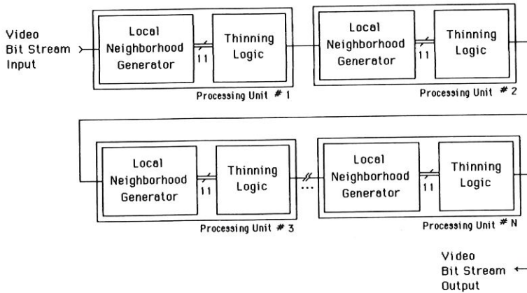
FIG. 9. A pipe containing processing devices for thinning iterations.
