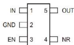
DBV Package 5-Pin SOT-23 Fixed Voltage Version Top View
