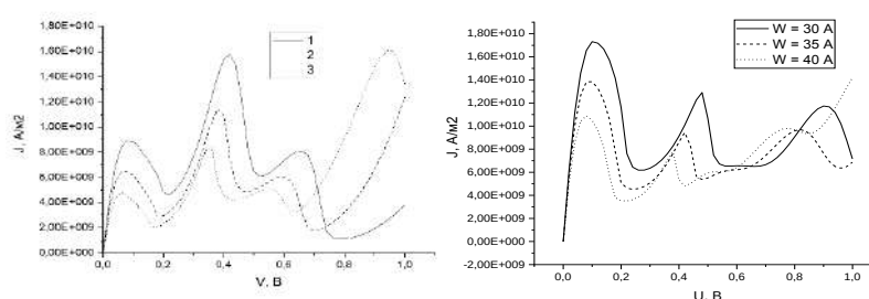
Figure 4 - Current-voltage characteristic at different values of the width of the quantum wells
