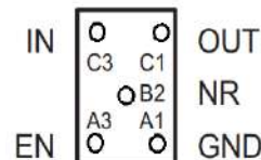
YZQ Package 5-Pin DSBGA Top View
