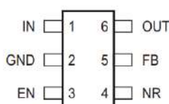
DBV Package 6-Pin SOT-23 Adjustable Voltage Version Top View
